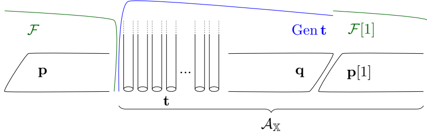
Figure 5.4: Auslander-Reiten quiver of the heart \mathcal{A}_{\mathbb{X}} = \mathcal{B}(\text{Gen } \mathbf{t}, \mathcal{F}) , for P = \mathbb{X} .
