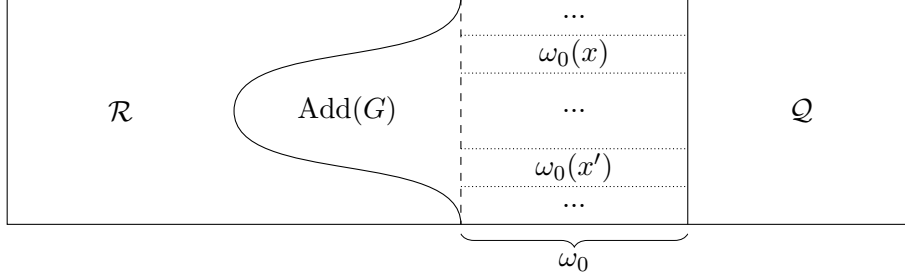
Figure 3.2: Subclasses of \text{Mod-}\Lambda .
