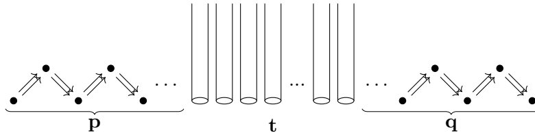
Figure 1: Auslander-Reiten quiver of the category of finite length modules over the Kronecker algebra.
