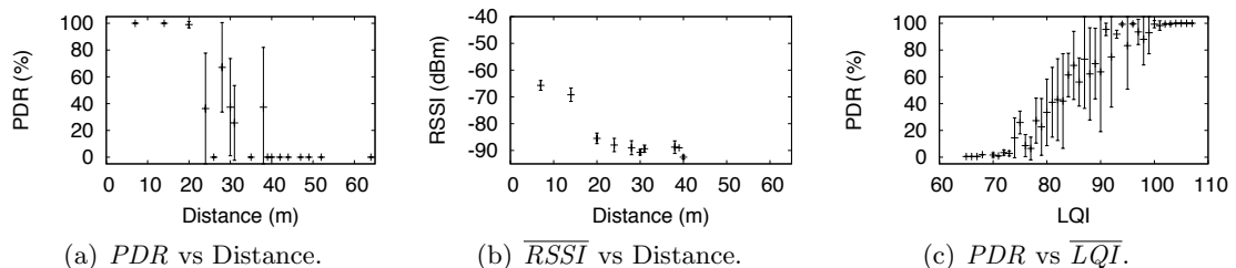
Figure 6.4: Average and standard deviation of the results from stationary tests with power -1 dBm.
