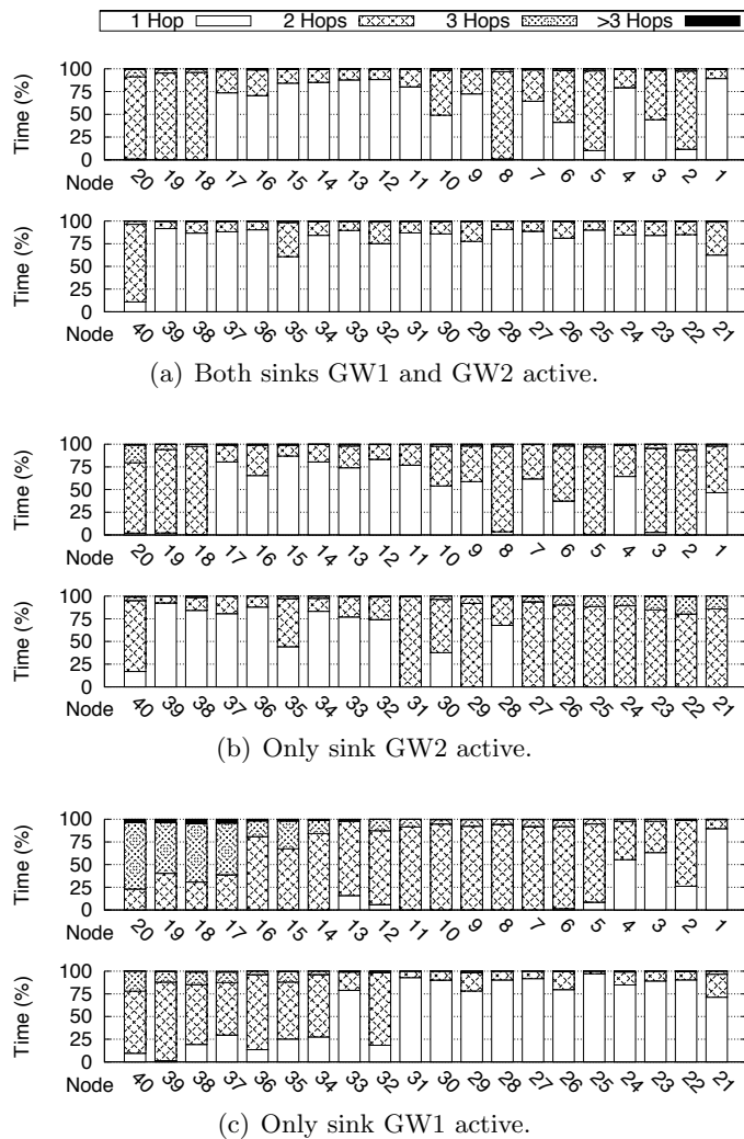
Figure 3.16: Percentage of time spent by each node at a given distance (hop count) from a sink.
