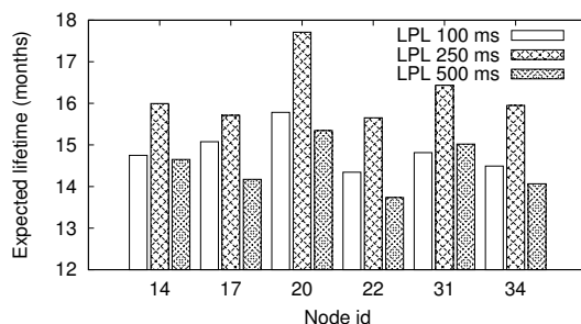
Figure 3.18: Expected lifetime, beyond one year.
