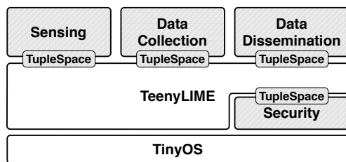
Figure 3.6: Software architecture.
