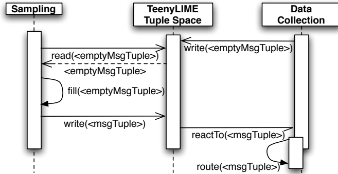
Figure 2.6: Handling sampled data over for routing.
