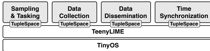
Figure 2.3: Software architecture.
