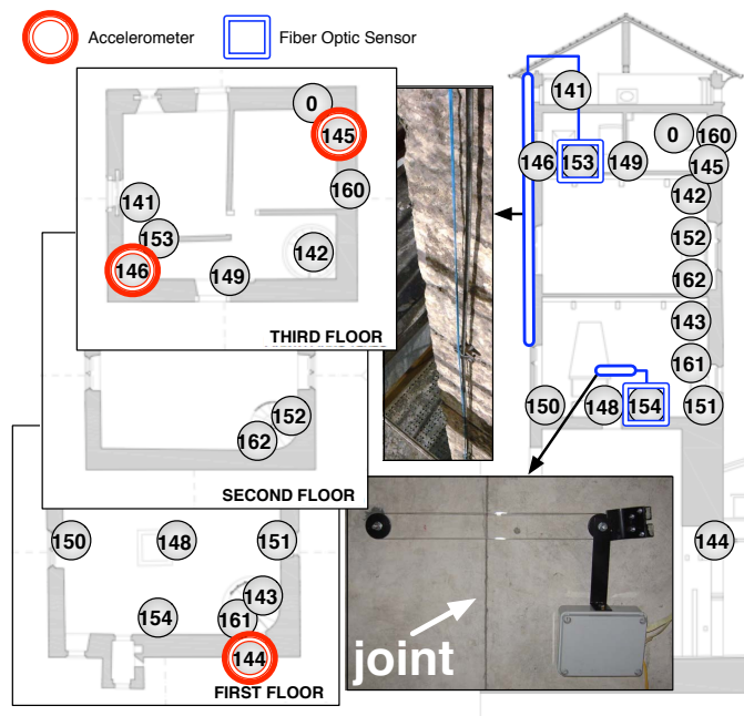
Figure 2.10: Deployment map.
